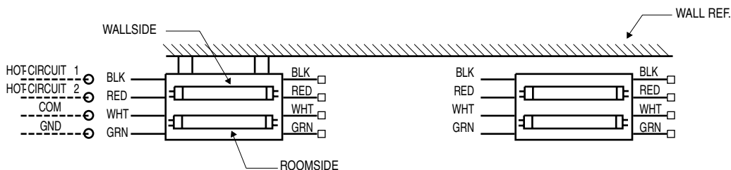
Wall-Mounted Fixtures Two-Circuit With Push-in Quick-Connects (2CWQ)
