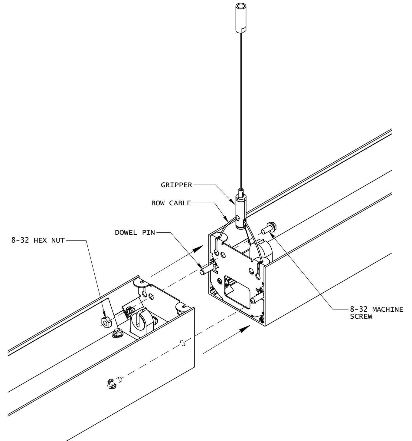
VIEW "D" - ROW JOINT ASSEMBLY
