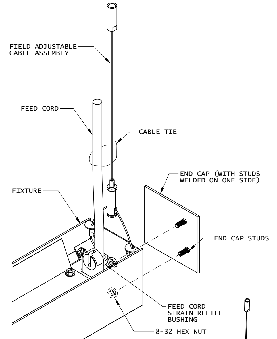
VIEW A
