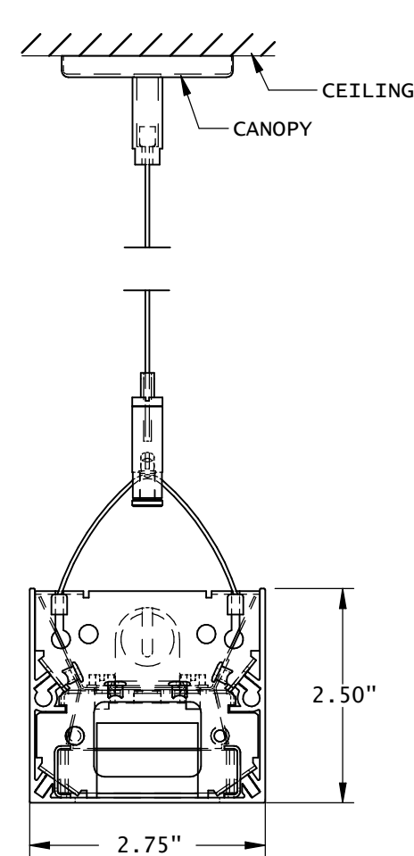
CROSS SECTION
