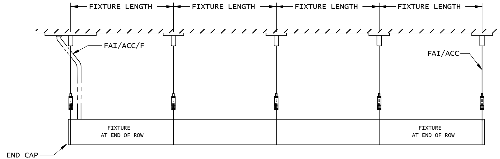
SIDE VIEW - ROW MOUNTED
