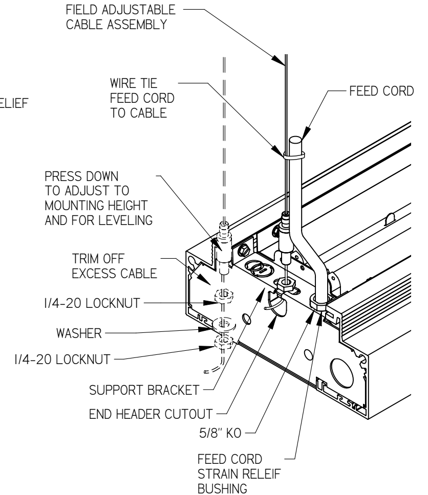
VIEW "D" PID82MS00 FIXTURE SHOWN
