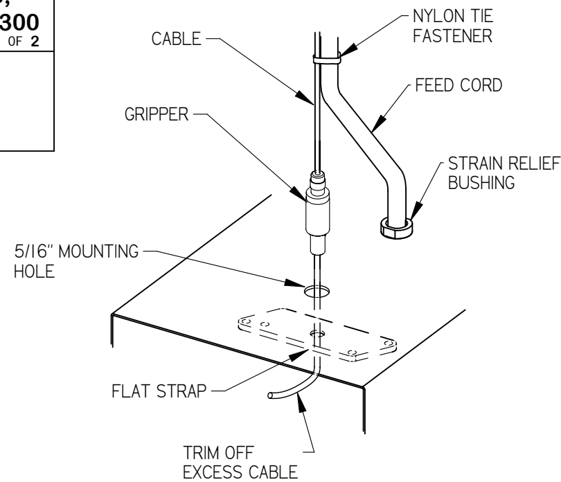
VIEW "C" PD-0200 FIXTURES
